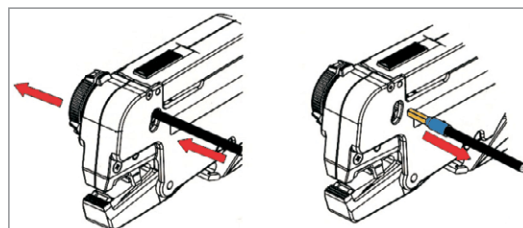
Terminal crimping
