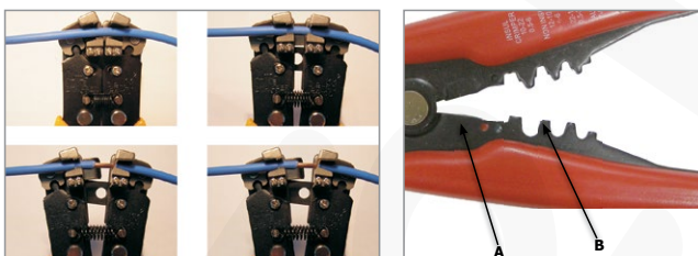
Insulation stripping
